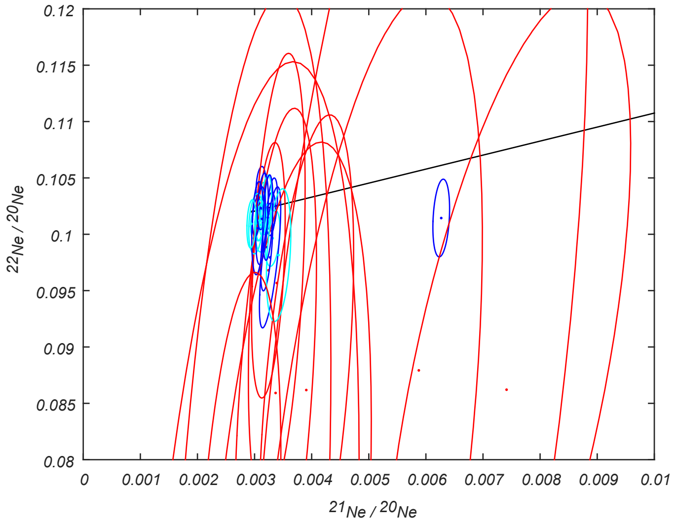
Figure S1b. Neon isotope ratios measured in Williams Hills quartz (see Table S3b). Ellipses show 68% confidence regions. Light blue, dark blue, and red data are low (400° C), intermediate (850° C) and high (1100° C) temperature steps, respectively. The black line is the mixing line between atmospheric-composition and cosmogenic Ne.
