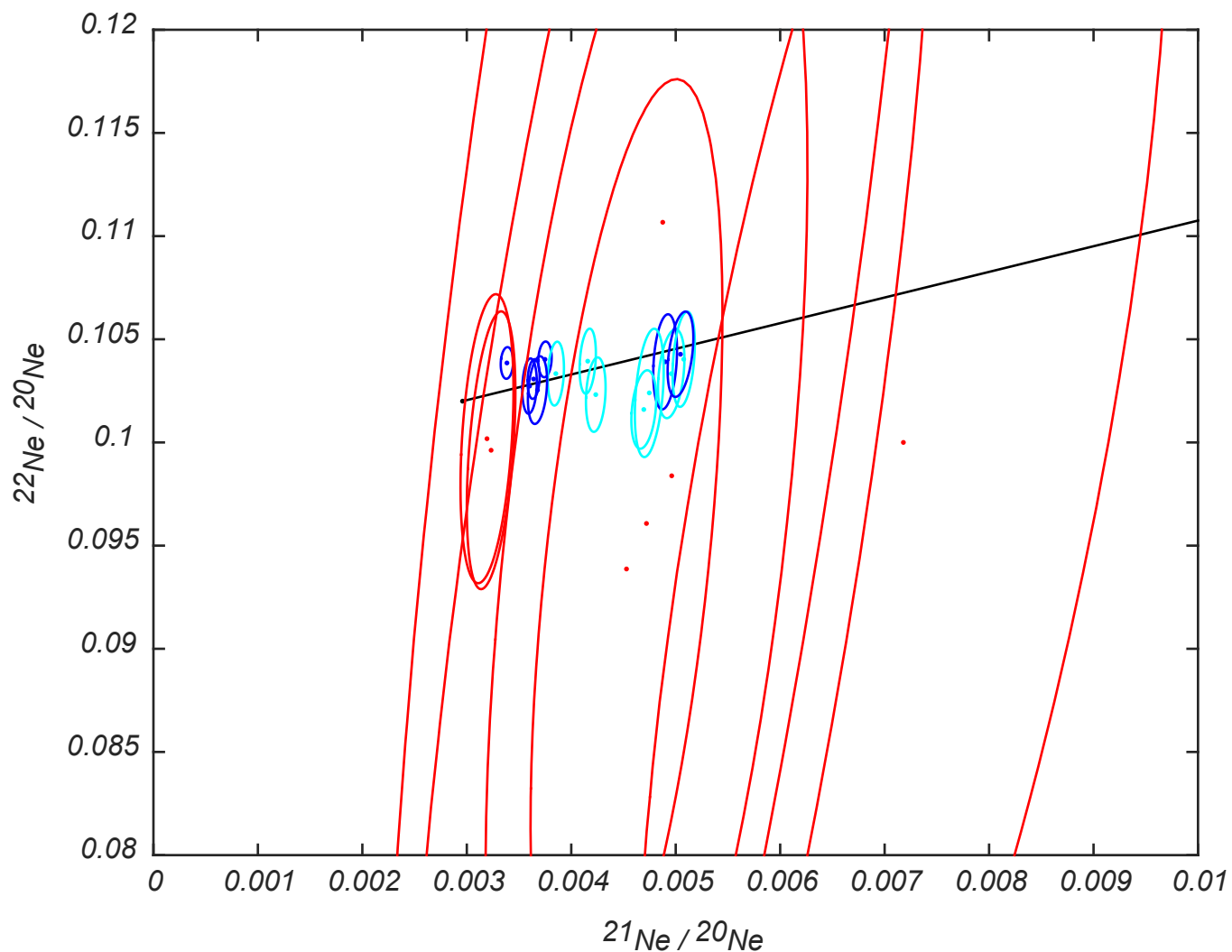
Figure S1c. Neon isotope ratios measured in quartz from Yarborough Till boulders (see Table S3c). Ellipses show 68% confidence regions. Light blue, dark blue, and red data are low (400° C), intermediate (850° C) and high (1100° C) temperature steps, respectively. The black line is the mixing line between atmospheric-composition and cosmogenic Ne.
