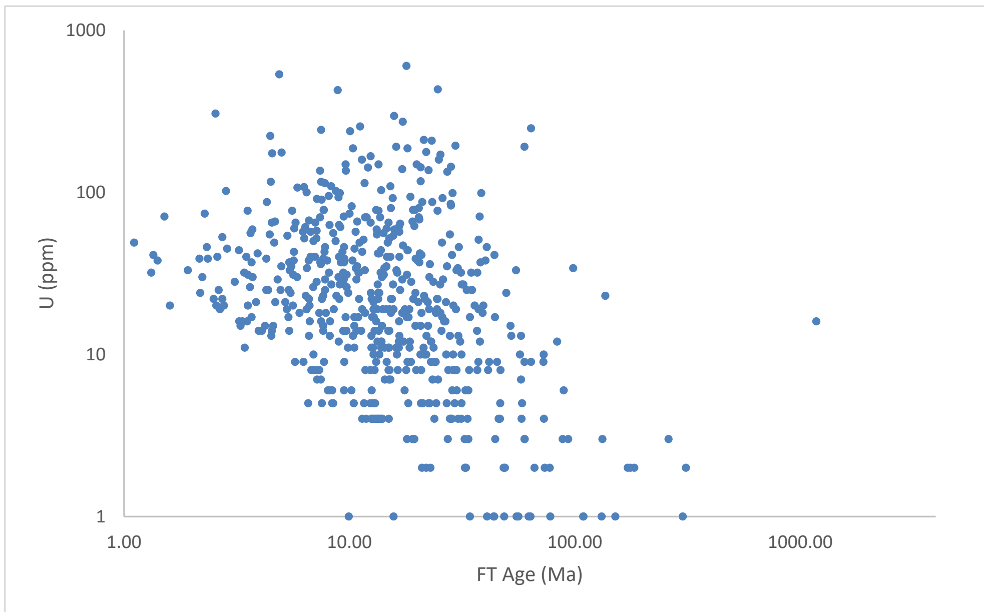
Fig SI 4b: plot showing relationship between U content and AFT ages for detrital grains
