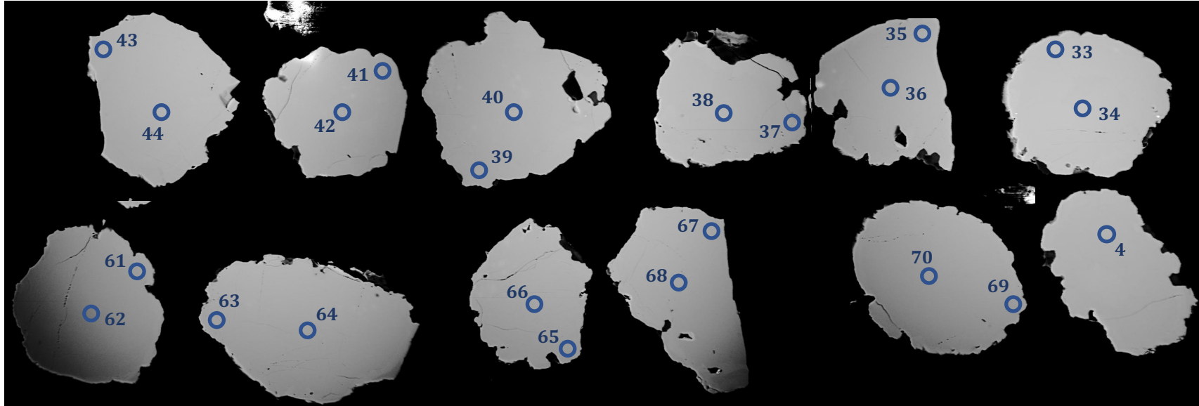
BSE images of B1550 titanite : group C framboidal textured / lenticular morphology
