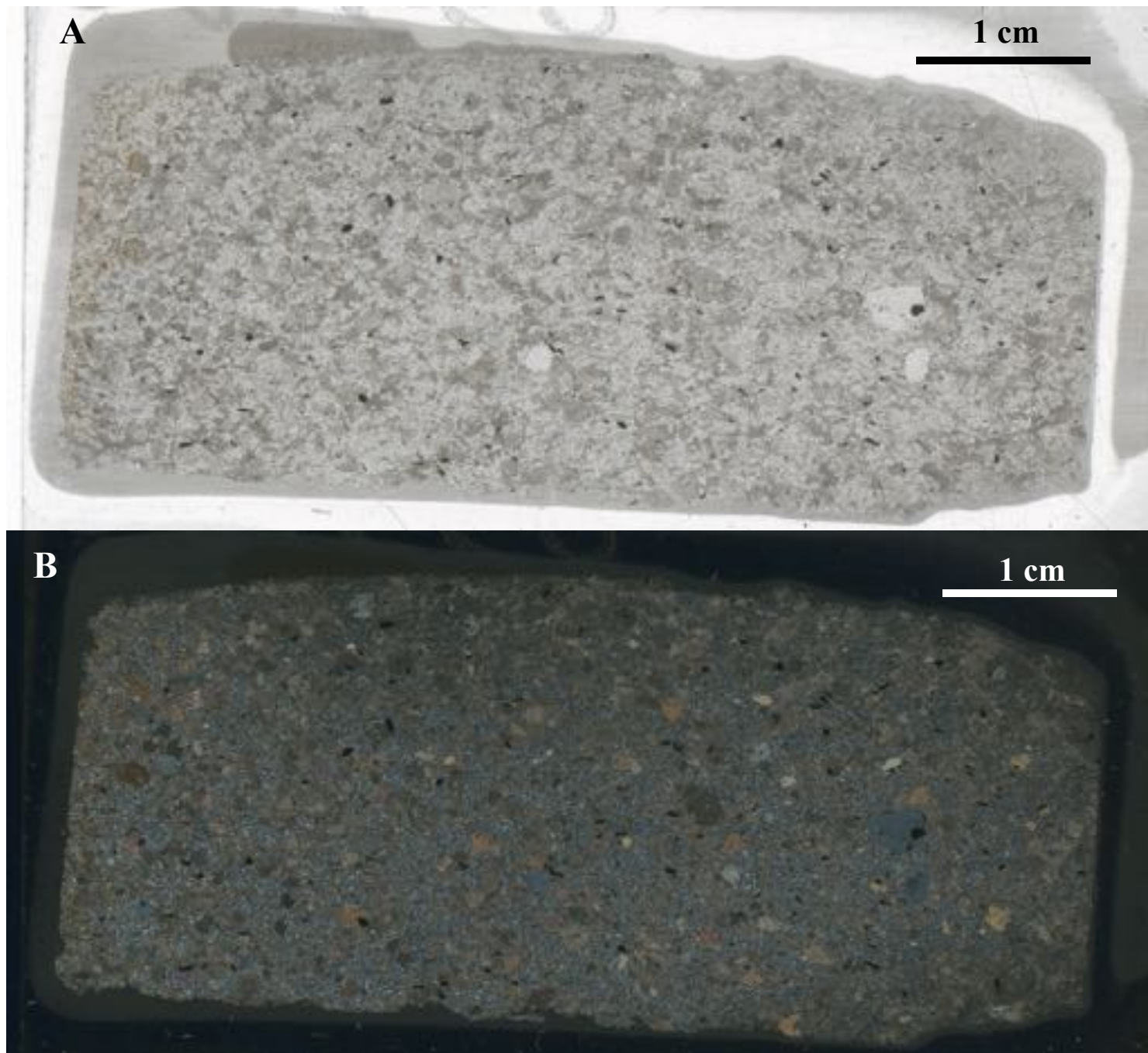
Figure S3: B1550 Mt Musgrave Gp Calcareous conglomerate Thin Section
